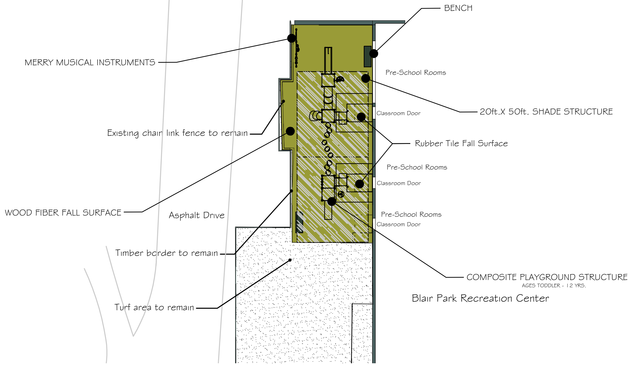
RECREATION CENTER PRE-SCHOOL PLAYGROUND CONCEPT PLAN scale 1" = 20ft.
